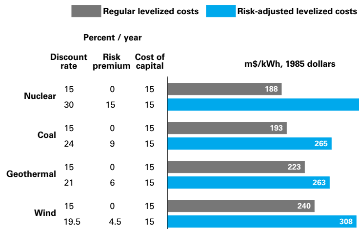
Figure 2-17: The importance of risk-adjusted discount rates Risk-adjusting plant comparisons can change their economic priority.
