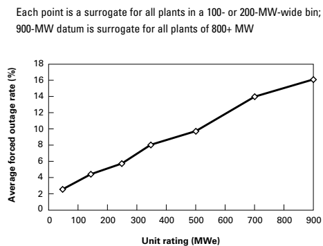
Figure 1-9: The forced-outage trap Bigger plants were proving less reliable.
