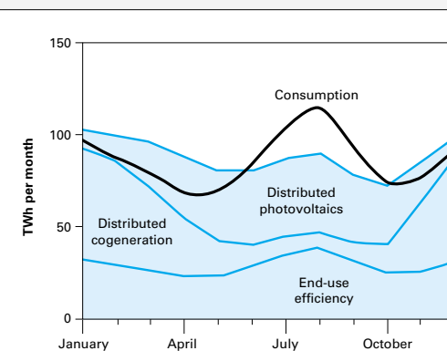
Figure 2-24a: Measured electricity consumption and estimated production using distributed resources (U.S. residential sector in 1995)
