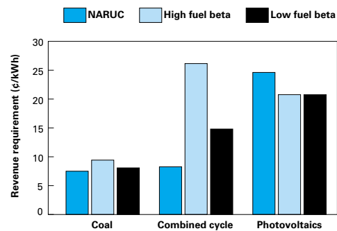
Figure 2-18: Fuel-price risk can dominate comparisons WACC discounting ignores fuel risks.
