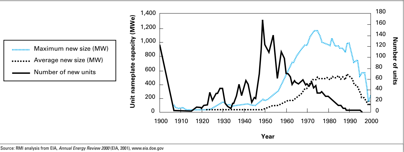
Figure 1-14: Maximum and average size of new generating units (fossil-fueled steam, all U.S. utilities, five-year rolling average) by year of entry into service
