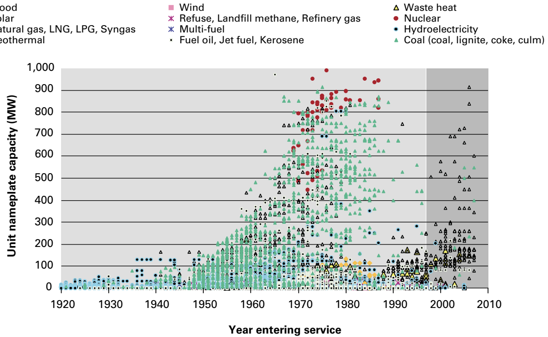
Figure 1-17: U.S. utility generating capacity commissioned 1920–2007
