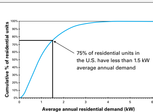
Figure 1-25: Average electricity demand of U.S. residential units, 1997
